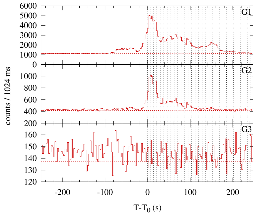
Konus-WIND S2 SOL2004-07-22T11:05 (C5.8) T_0 = 39907.387 s UT (11:05:07.387)
