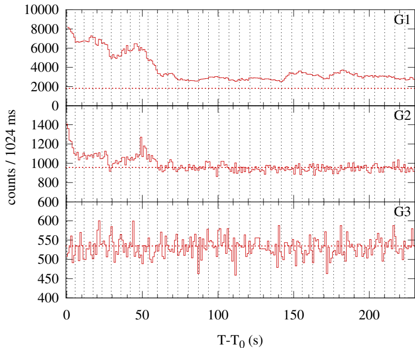
Konus-WIND S2 SOL2004-07-23T21:19 (M1.7) T 0 = 76764.33 s UT (21:19:24.33)
