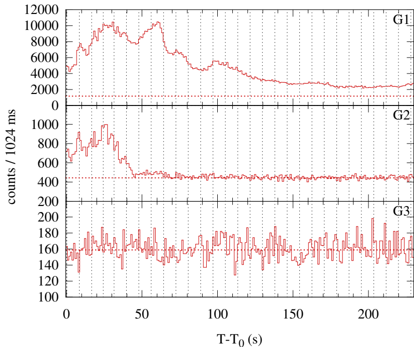
Konus-WIND S2 SOL2004-07-24T18:44 (M2.5) T_0 = 67467.795 s UT (18:44:27.795)
