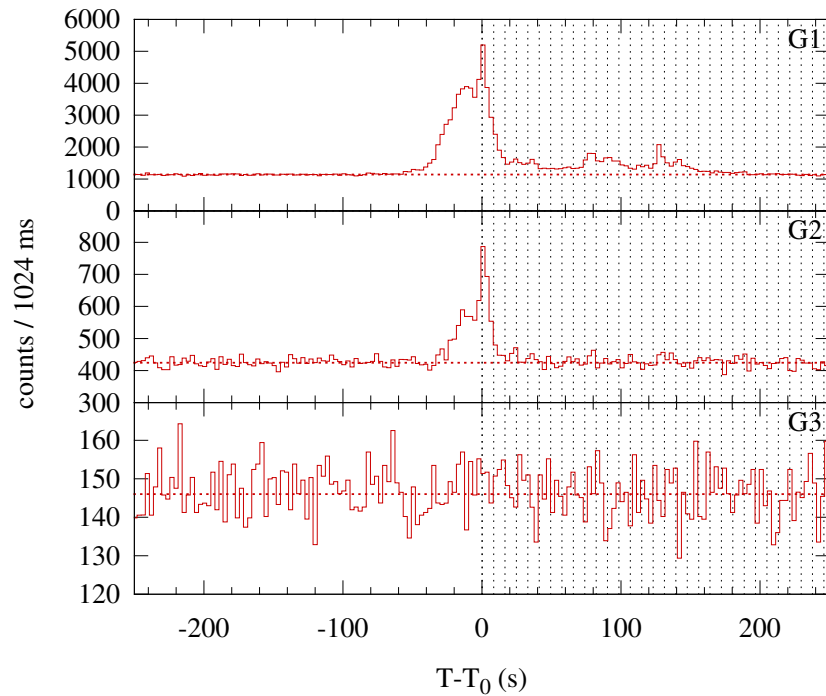
Konus-WIND S2 SOL2004-07-25T00:28 (C7.4) T 0 = 1734.446 s UT (00:28:54.446)
