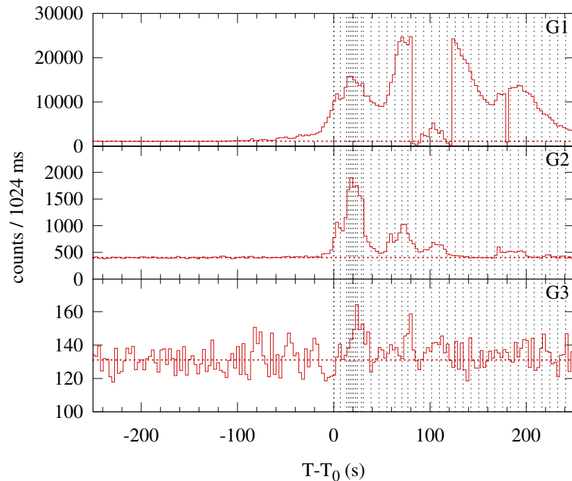
Konus-WIND S2 SOL2004-08-13T18:09 (X1.0) T_0 = 65393.526 s UT (18:09:53.526)
