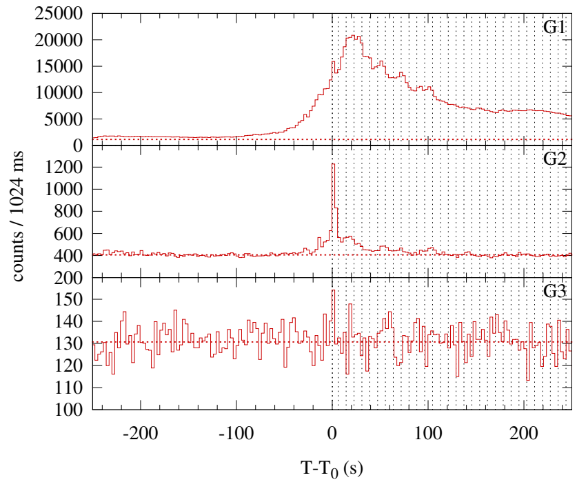
Konus-WIND S2 SOL2004-08-14T05:43 (M7.4) T_0 = 20591.59 s UT (05:43:11.59)
