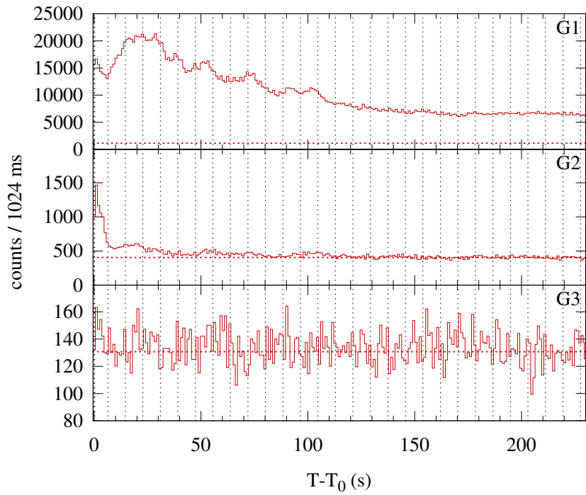
Konus-WIND S2 SOL2004-08-14T05:43 (M7.4) T_0 = 20591.59 s UT (05:43:11.59)
