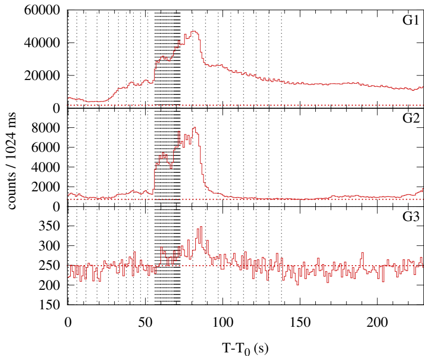
Konus-WIND S2 SOL2004-10-30T11:42 (X1.2) T_0 = 42162.638 s UT (11:42:42.638)
