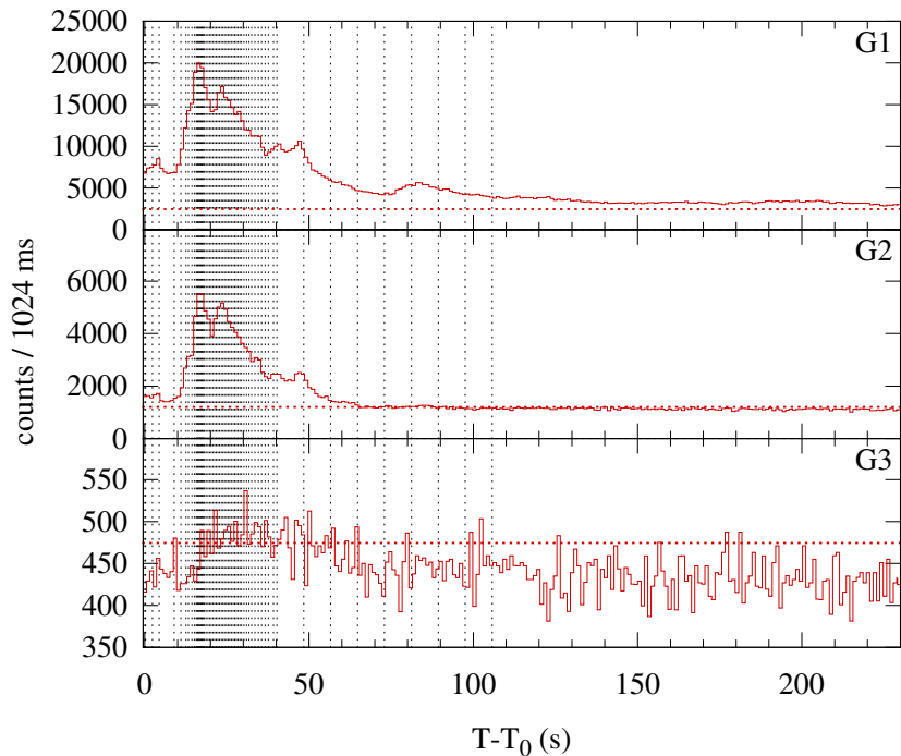
Konus-WIND S2 SOL2004-10-30T16:24 (M5.9) T 0 = 59043.637 s UT (16:24:03.637)
