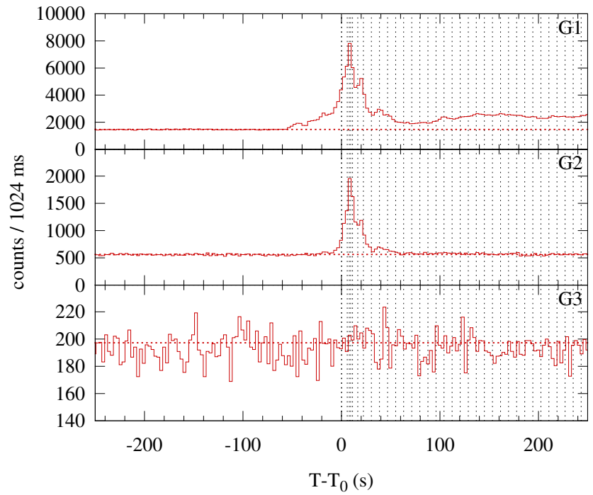
Konus-WIND S2 SOL2004-10-31T05:26 (M2.3) T_0 = 19598.860 s UT (05:26:38.860)
