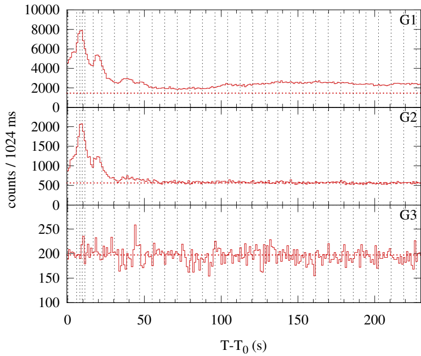
Konus-WIND S2 SOL2004-10-31T05:26 (M2.3) T_0 = 19598.860 s UT (05:26:38.860)
