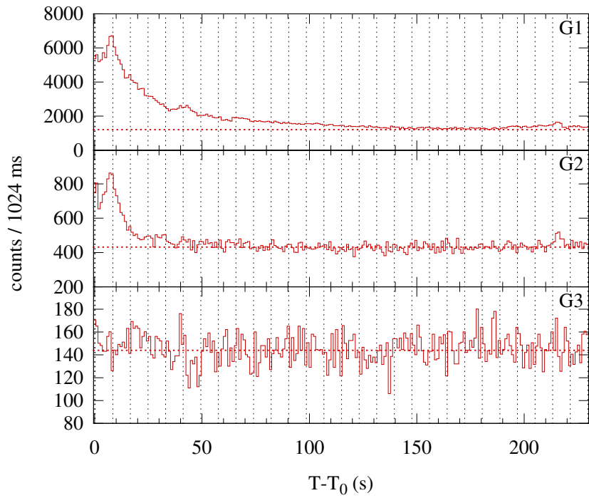
Konus-WIND S2 SOL2004-11-01T03:18 (M1.1) T_0 = 11933.505 s UT (03:18:53.505)
