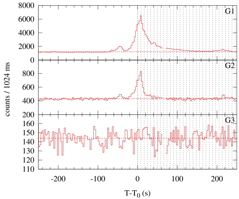
Konus-WIND S2 SOL2004-11-01T03:18 (M1.1) T_0 = 11933.505 s UT (03:18:53.505)
