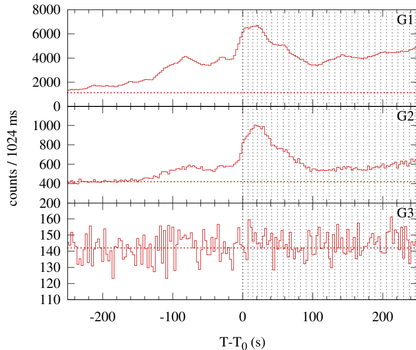
Konus-WIND S2 SOL2004-11-04T22:54 (M5.4) T 0 = 82478.116 s UT (22:54:38.116)
