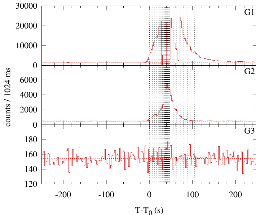
Konus-WIND S2 SOL2004-11-05T11:28 (M4.0) T 0 = 41301.423 s UT (11:28:21.423)
