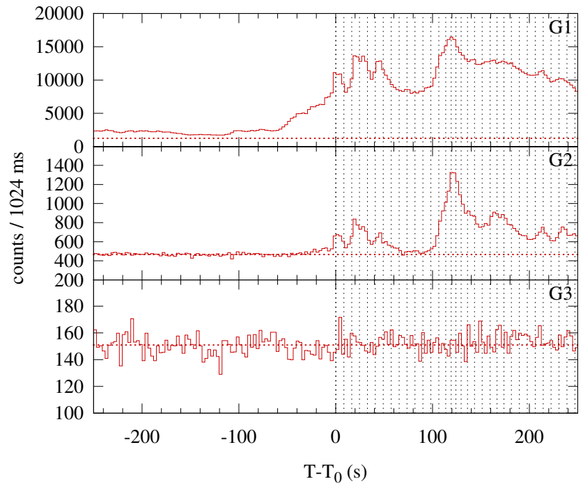
Konus-WIND S2 SOL2004-11-06T00:28 (M9.3) T_0 = 1726.571 s UT (00:28:46.571)
