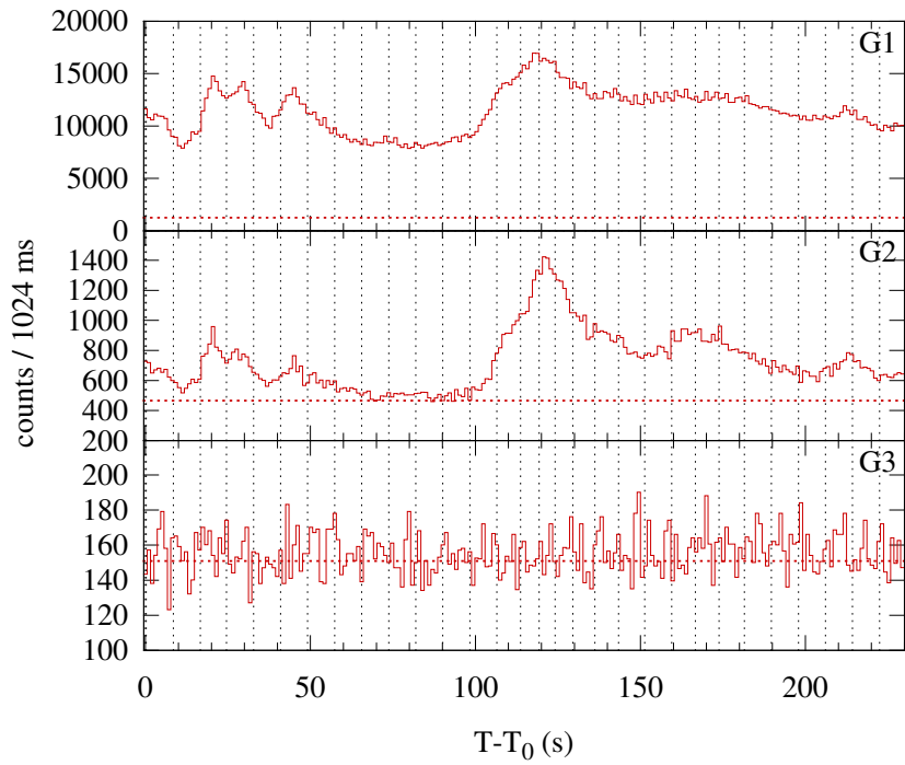
Konus-WIND S2 SOL2004-11-06T00:28 (M9.3) T_0 = 1726.571 s UT (00:28:46.571)
