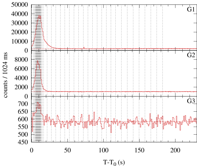
Konus-WIND S2 SOL2004-11-08T15:45 (M2.3) T 0 = 56756.459 s UT (15:45:56.459)
