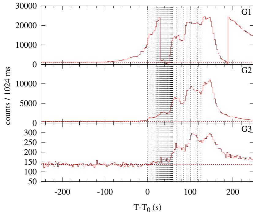
Konus-WIND S2 SOL2005-01-01T00:27 (X1.7) T_0 = 1657.406 s UT (00:27:37.406)
