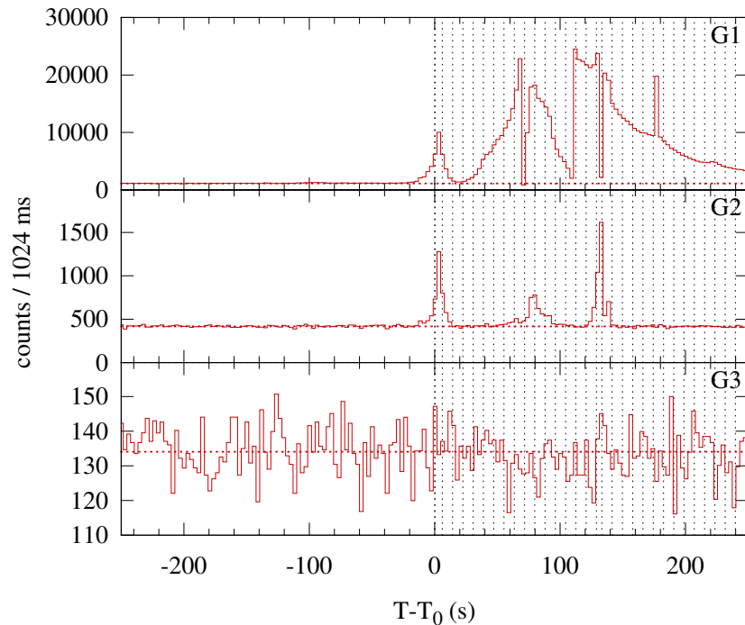
Konus-WIND S2 SOL2005-01-15T04:28 (M8.4) T_0 = 16123.804 s UT (04:28:43.804)
