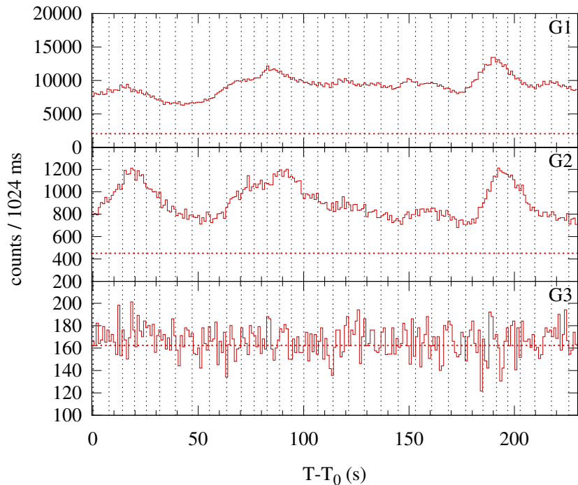
Konus-WIND S2 SOL2005-01-15T22:32 (X2.6) T_0 = 81163.160 s UT (22:32:43.160)
