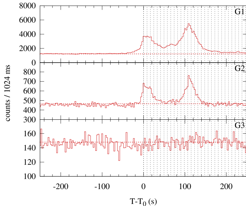
Konus-WIND S2 SOL2005-05-05T20:13 (C7.8) T_0 = 72830.849 s UT (20:13:50.849)
