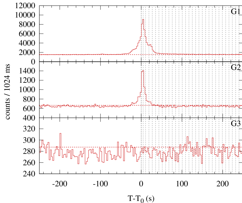
Konus-WIND S2 SOL2005-07-14T06:04 (M9.1) T 0 = 21850.813 s UT (06:04:10.813)
