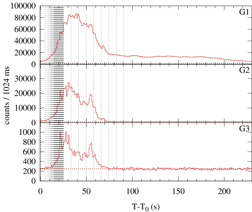
Konus-WIND S2 SOL2005-07-14T07:22 (M9.1) T_0 = 26546.308 s UT (07:22:26.308)
