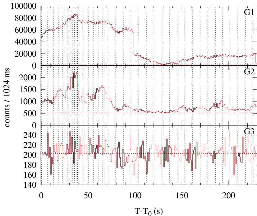
Konus-WIND S2 SOL2005-09-07T17:25 (X17.0) T_0 = 62717.585 s UT (17:25:17.585)
