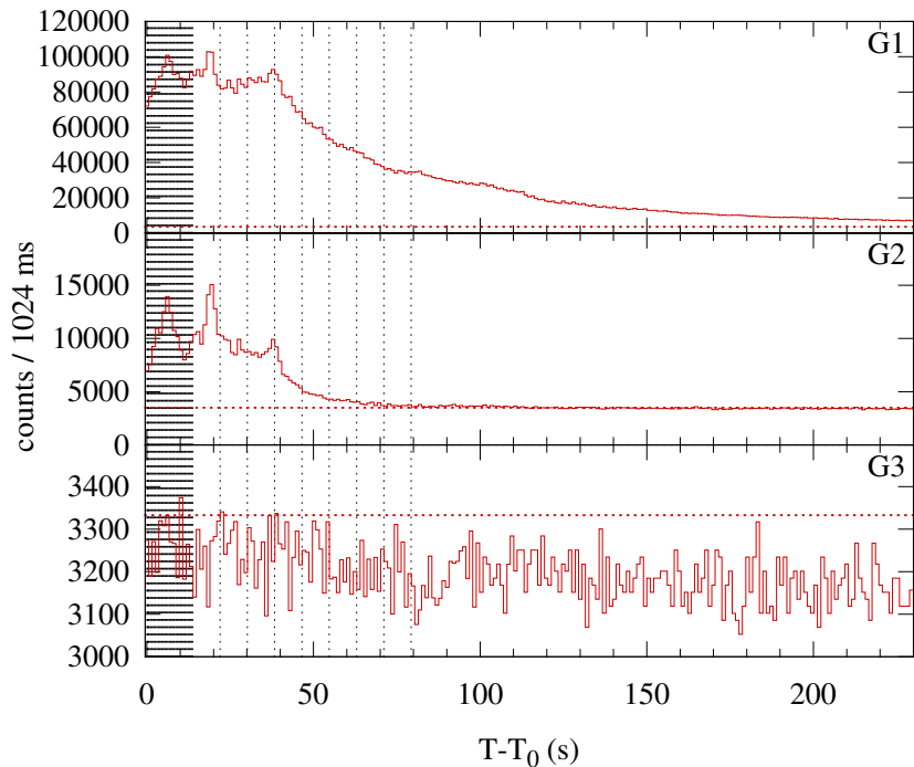
Konus-WIND S2 SOL2005-09-15T08:35 (X1.1) T_0 = 30958.579 s UT (08:35:58.579)
