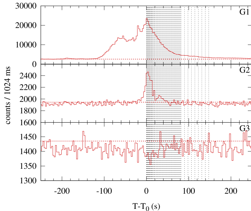
Konus-WIND S2 SOL2005-09-16T01:47 (M4.4) T_0 = 6452.651 s UT (01:47:32.651)
