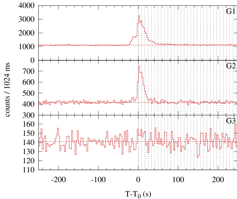
Konus-WIND S2 SOL2006-01-05T09:20 (C4.4) T_0 = 33625.107 s UT (09:20:25.107)
