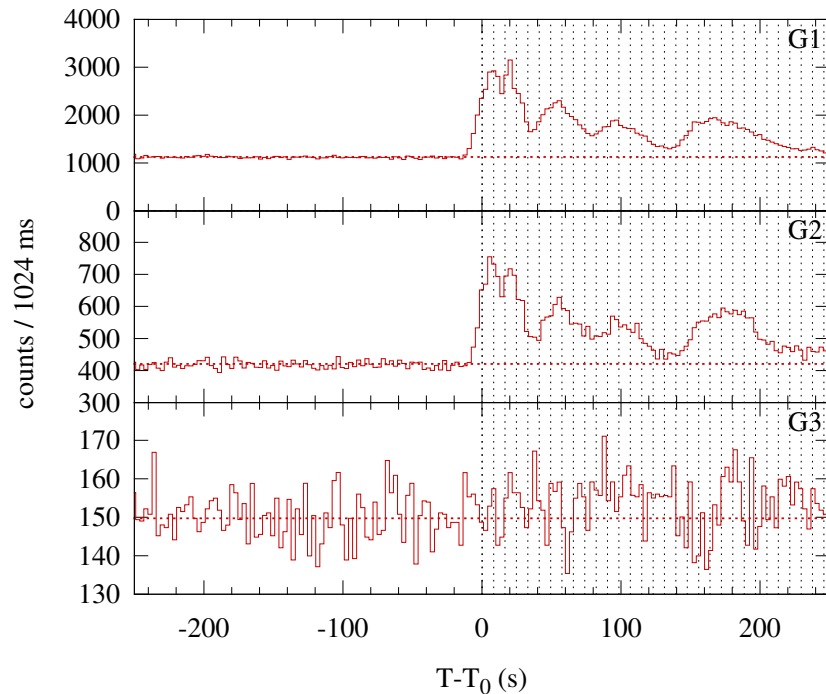
Konus-WIND S2 SOL2006-04-30T01:53 (C5.3) T_0 = 6790.624 s UT (01:53:10.624)
