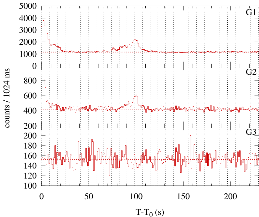
Konus-WIND S2 SOL2006-08-15T10:42 (B8.1) T 0 = 38569.468 s UT (10:42:49.468)
