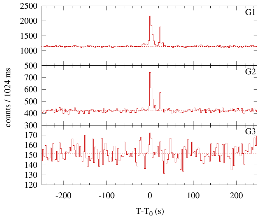
Konus-WIND S2 SOL2006-08-28T11:04 (C1.8) T 0 = 39841.314 s UT (11:04:01.314)
