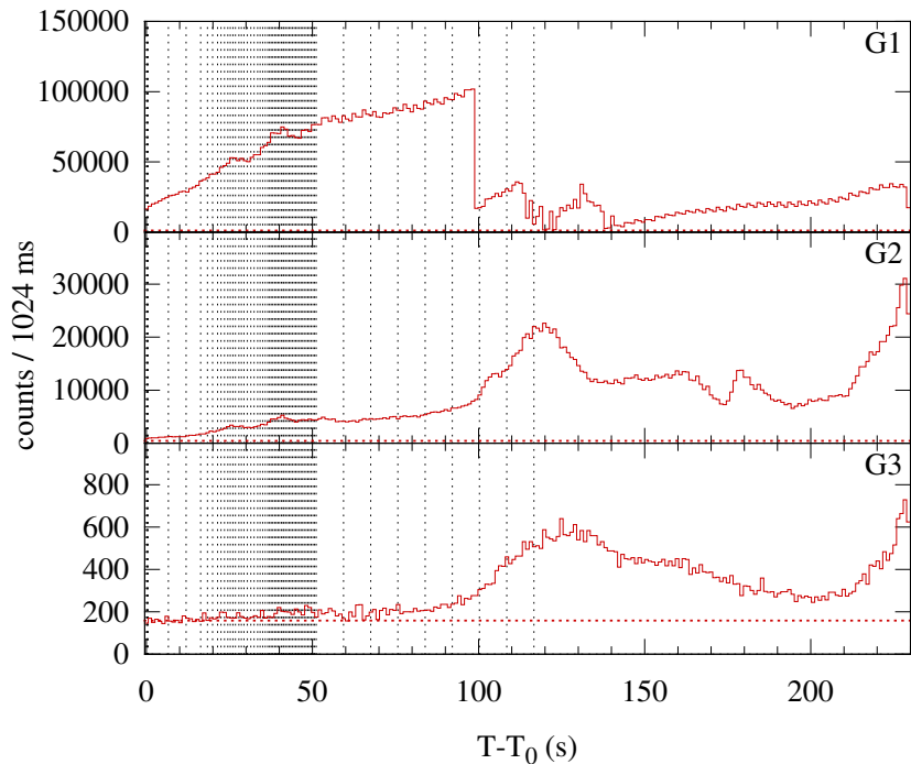
Konus-WIND S2 SOL2006-12-05T10:26 (X9.0) T 0 = 37563.142 s UT (10:26:03.142)
