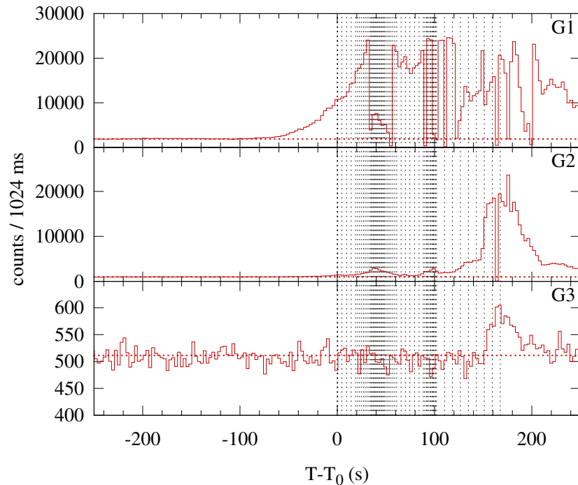
Konus-WIND S2 SOL2006-12-13T02:22 (X3.4) T_0 = 8536.577 s UT (02:22:16.577)
