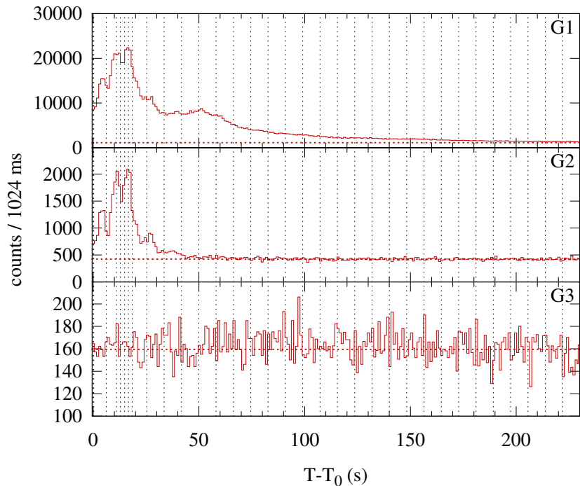
Konus-WIND S2 SOL2007-06-01T21:49 (M2.1) T_0 = 78571.977 s UT (21:49:31.977)
