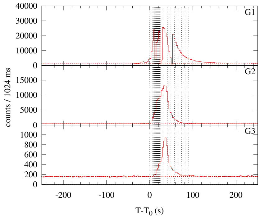
Konus-WIND S2 SOL2007-06-03T06:39 (M4.5) T_0 = 23955.63 s UT (06:39:15.63)
