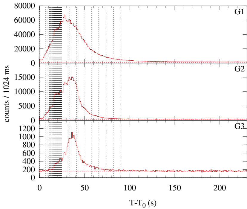
Konus-WIND S2 SOL2007-06-03T06:39 (M4.5) T_0 = 23955.63 s UT (06:39:15.63)
