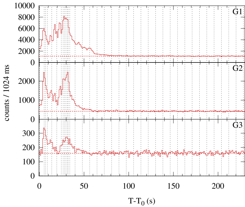
Konus-WIND S2 SOL2007-06-03T09:26 (C5.3) T_0 = 33990.426 s UT (09:26:30.426)
