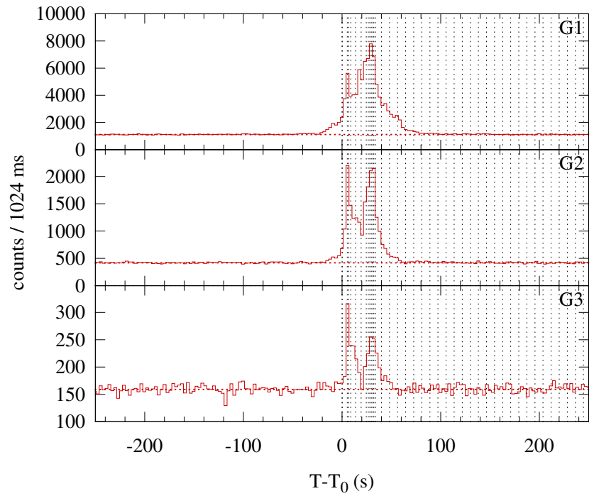
Konus-WIND S2 SOL2007-06-03T09:26 (C5.3) T_0 = 33990.426 s UT (09:26:30.426)
