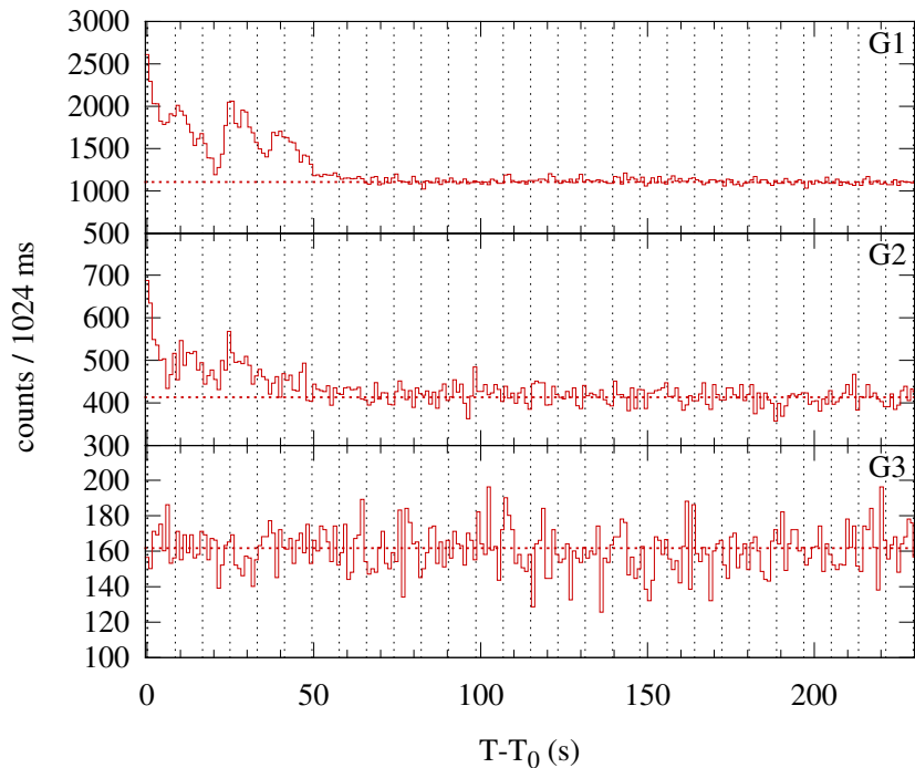
Konus-WIND S2 SOL2011-02-14T19:29 (C6.6) T_0 = 70160.77 s UT (19:29:20.77)
