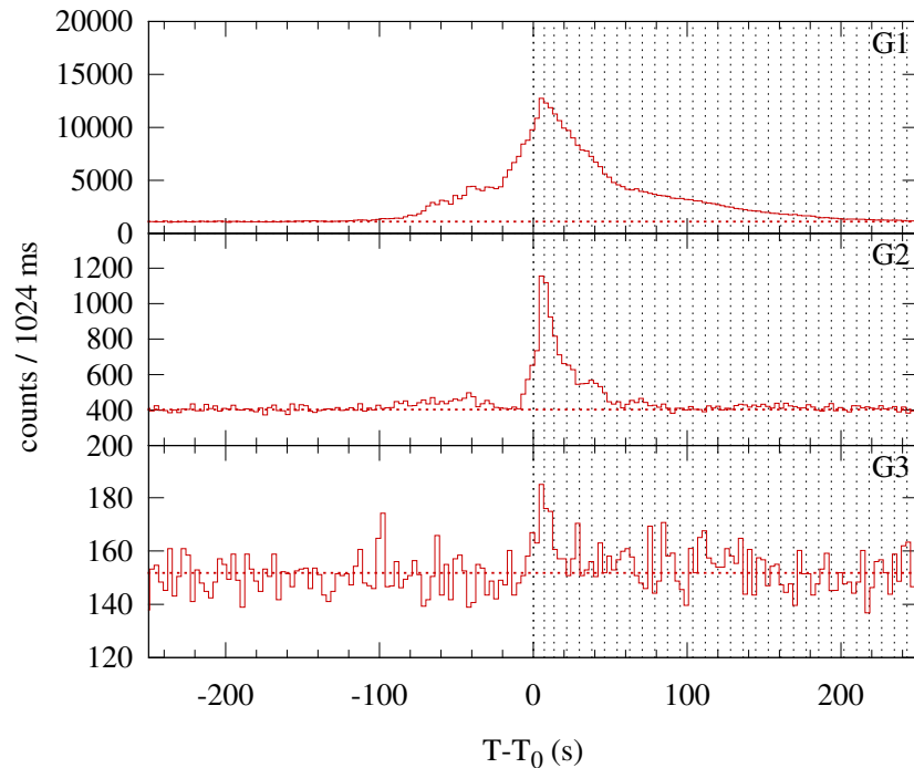
Konus-WIND S2 SOL2011-02-18T10:10 (M6.6) T_0 = 36648.442 s UT (10:10:48.442)
