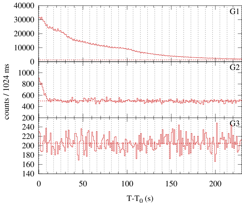
Konus-WIND S2 SOL2011-03-09T23:21 (X1.5) T_0 = 84070.759 s UT (23:21:10.759)
