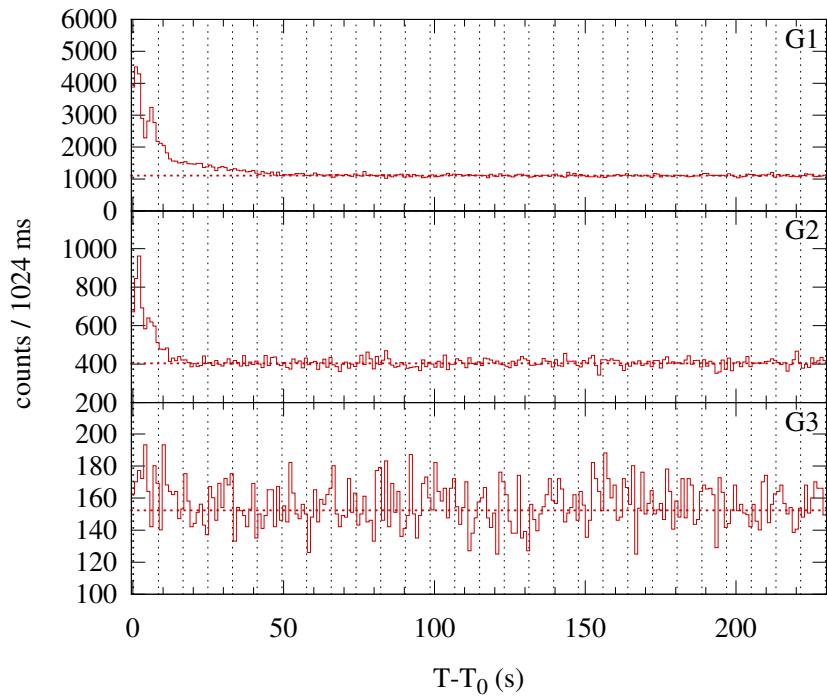
Konus-WIND S2 SOL2011-03-15T00:21 (M1.0) T 0 = 1317.533 s UT (00:21:57.533)
