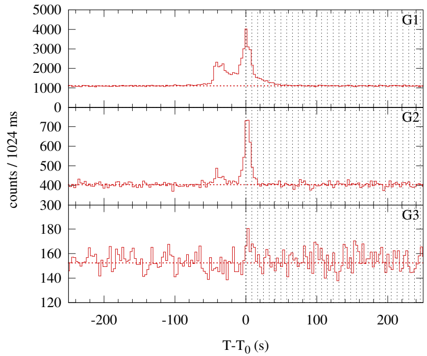
Konus-WIND S2 SOL2011-03-15T00:21 (M1.0) T 0 = 1317.533 s UT (00:21:57.533)
