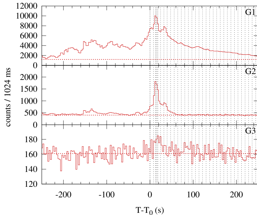
Konus-WIND S2 SOL2011-09-08T15:42 (M6.7) T 0 = 56572.314 s UT (15:42:52.314)
