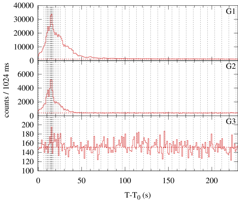
Konus-WIND S2 SOL2011-09-28T12:29 (C9.3) T 0 = 44942.43 s UT (12:29:02.43)
