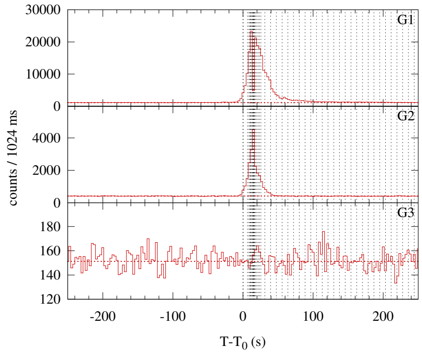
Konus-WIND S2 SOL2011-09-28T12:29 (C9.3) T 0 = 44942.43 s UT (12:29:02.43)
