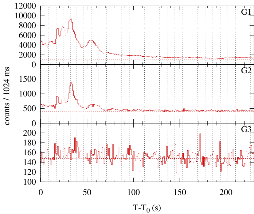
Konus-WIND S2 SOL2011-12-25T18:14 (M4.0) T_0 = 65659.917 s UT (18:14:19.917)
