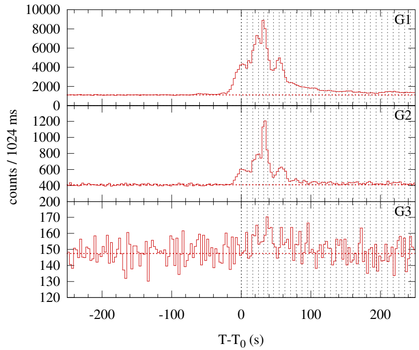
Konus-WIND S2 SOL2011-12-25T18:14 (M4.0) T_0 = 65659.917 s UT (18:14:19.917)
