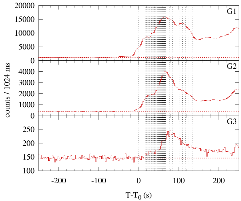
Konus-WIND S2 SOL2012-01-23T03:39 (M8.7) T_0 = 13161.544 s UT (03:39:21.544)
