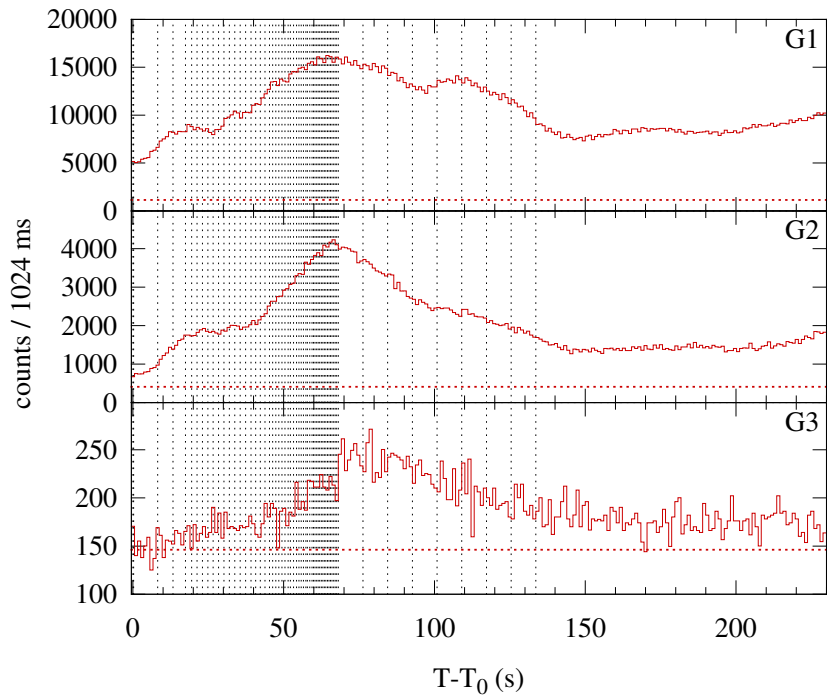
Konus-WIND S2 SOL2012-01-23T03:39 (M8.7) T_0 = 13161.544 s UT (03:39:21.544)
