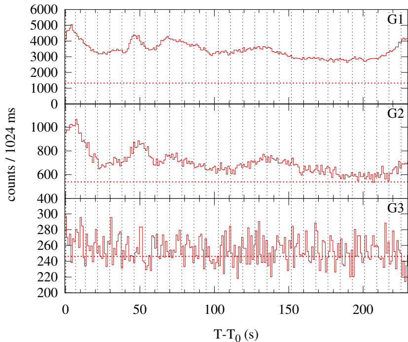
Konus-WIND S2 SOL2012-01-27T18:10 (X1.7) T 0 = 65447.139 s UT (18:10:47.139)
