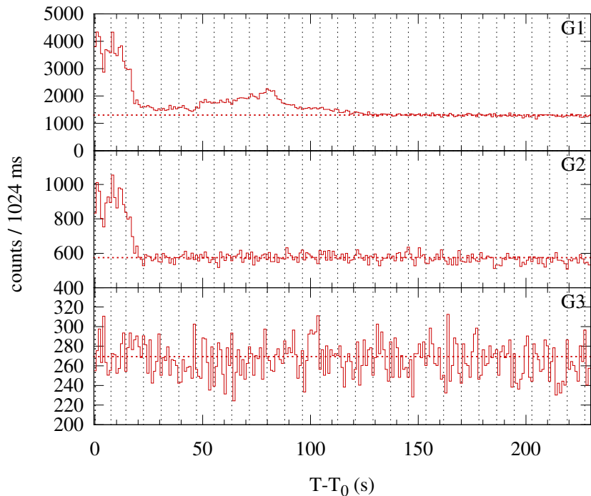
Konus-WIND S2 SOL2012-03-05T18:35 (C6.8) T 0 = 66932.267 s UT (18:35:32.267)
