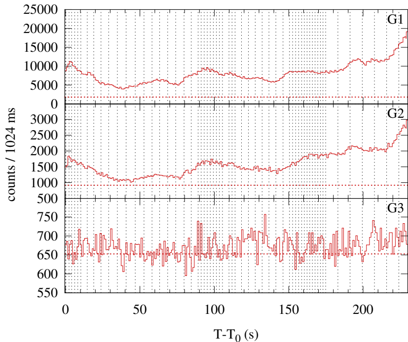
Konus-WIND S2 SOL2012-03-13T17:18 (M7.9) T_0 = 62310.275 s UT (17:18:30.275)
