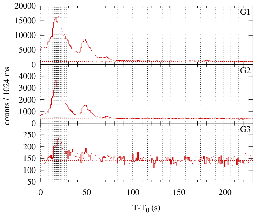
Konus-WIND S2 SOL2012-06-03T17:52 (M3.3) T_0 = 64377.92 s UT (17:52:57.92)
