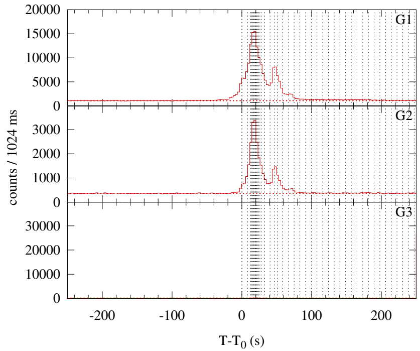
Konus-WIND S2 SOL2012-06-03T17:52 (M3.3) T_0 = 64377.92 s UT (17:52:57.92)
