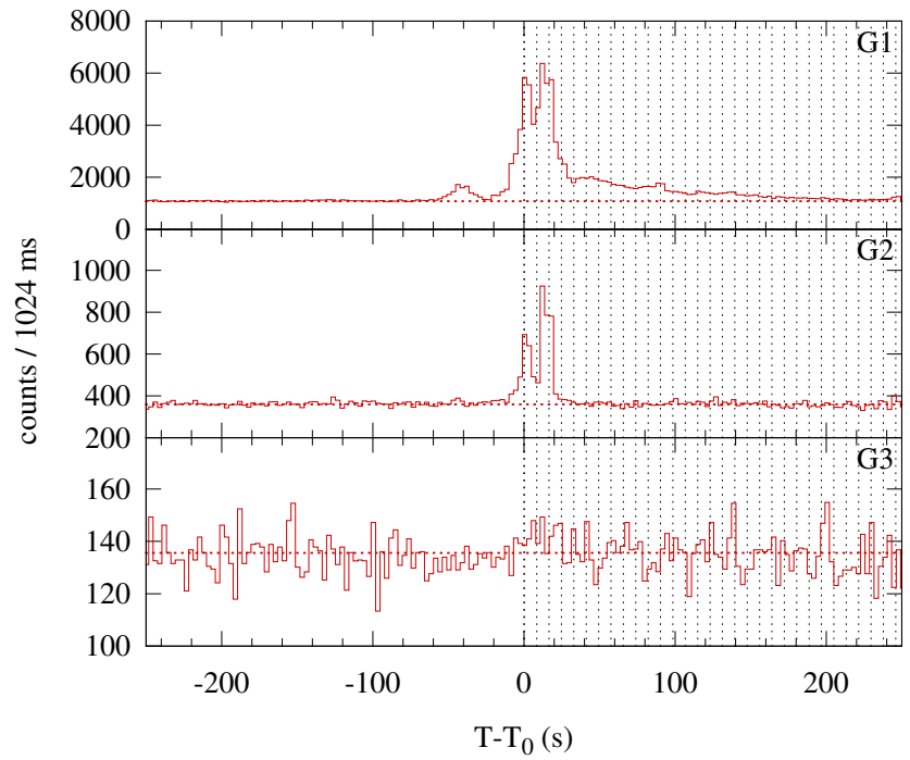
Konus-WIND S2 SOL2012-07-05T20:12 (M1.6) T_0 = 72766.372 s UT (20:12:46.372)
