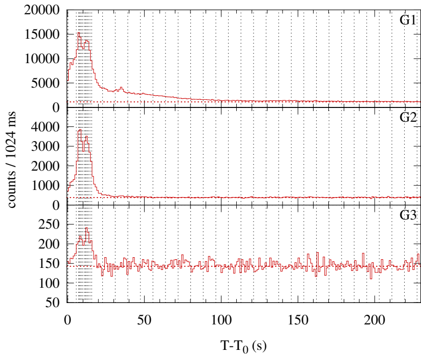
Konus-WIND S2 SOL2012-07-06T01:38 (M2.9) T 0 = 5917.394 s UT (01:38:37.394)
