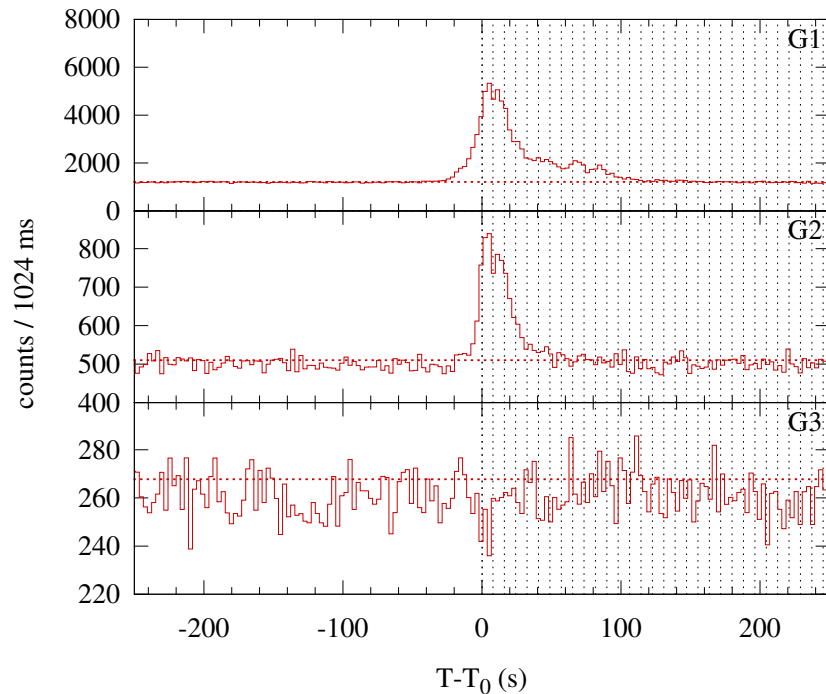
Konus-WIND S2 SOL2012-07-10T03:39 (C3.9) T_0 = 13180.476 s UT (03:39:40.476)
