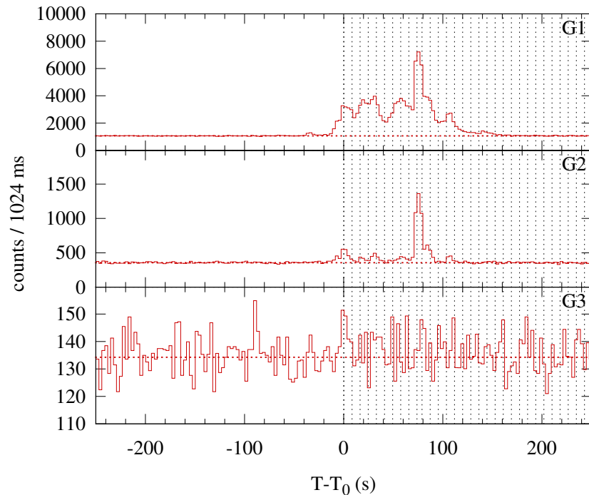
Konus-WIND S2 SOL2012-08-18T16:05 (M2.0) T 0 = 57954.470 s UT (16:05:54.470)
