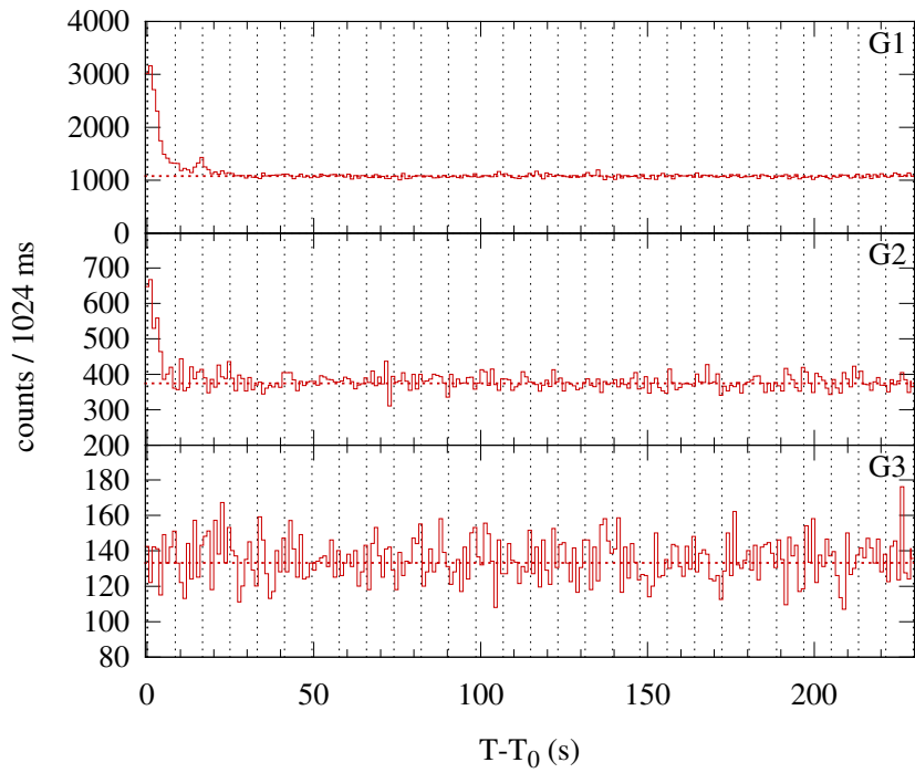
Konus-WIND S2 SOL2013-04-21T05:13 (C1.4) T 0 = 18783.606 s UT (05:13:03.606)
