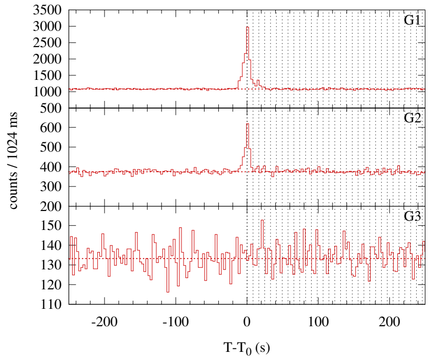
Konus-WIND S2 SOL2013-04-21T05:13 (C1.4) T 0 = 18783.606 s UT (05:13:03.606)
