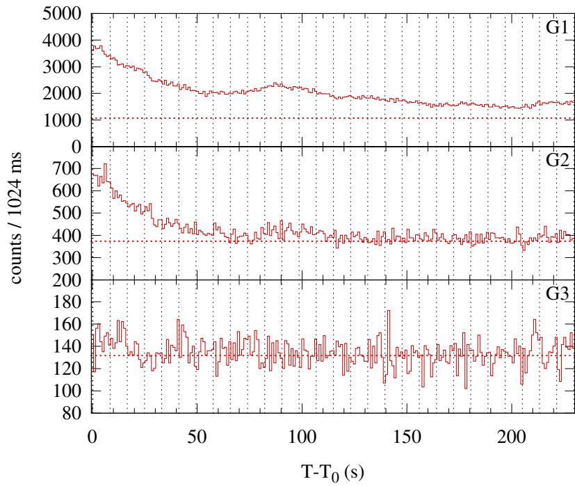
Konus-WIND S2 SOL2013-05-03T17:29 (M5.7) T 0 = 62981.651 s UT (17:29:41.651)
