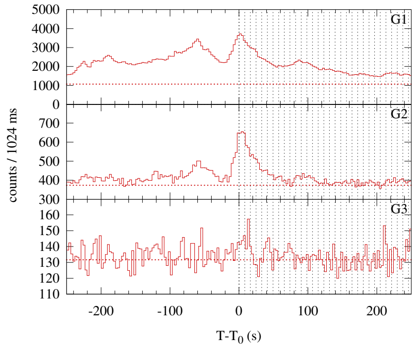
Konus-WIND S2 SOL2013-05-03T17:29 (M5.7) T 0 = 62981.651 s UT (17:29:41.651)
